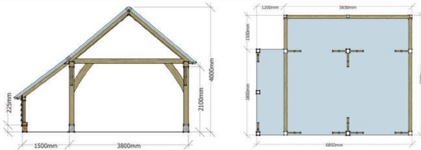
Dimensions for The Piltdown 2 Bay Garage Model A2-533L
