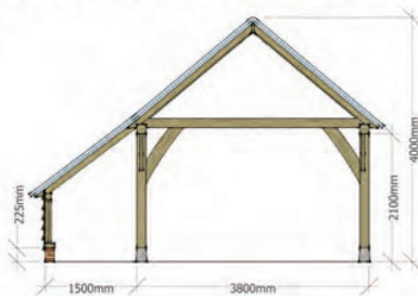
Dimensions for The Barcombe 2 Bay Garage Model A2-531
