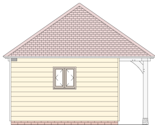
Left Hand Elevation
