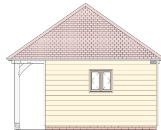
Right Hand Elevation
